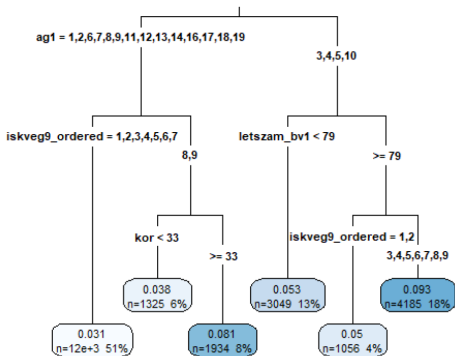
Figure 3.3 CART for 2010
