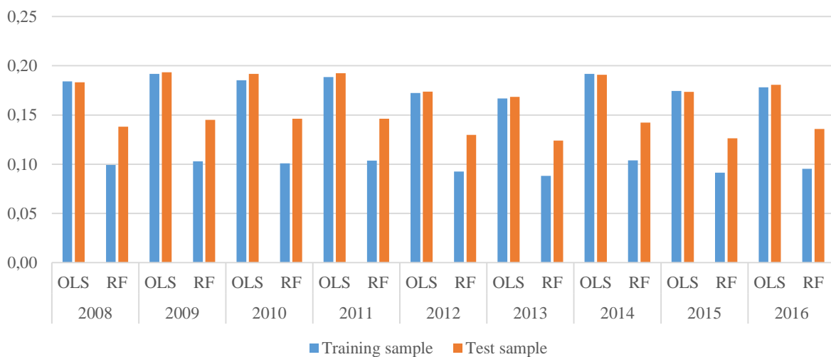
Figure 1 Comparison of predictive performance of OLS and Random Forest
