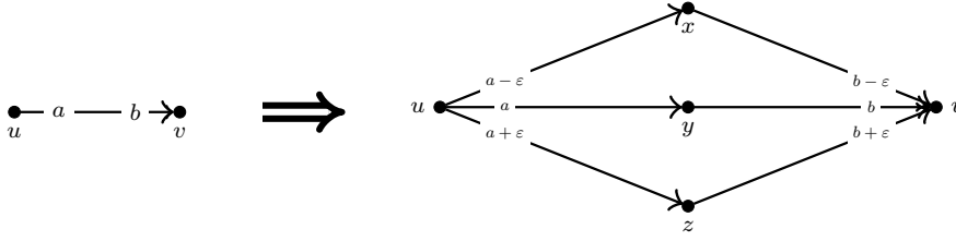
Fig. 4 Splitting an edge with lower and upper bounds. Due to the preferences, capacities and bounds defined on the modified instance, the first l(uv) units of flow will saturate \langle u, x, v \rangle , then, the coming u(uv) - l(uv) units of flow will saturate \langle u, y, v \rangle , and the remaining c(uv) - u(uv) units of flow will use \langle u, z, v \rangle .
