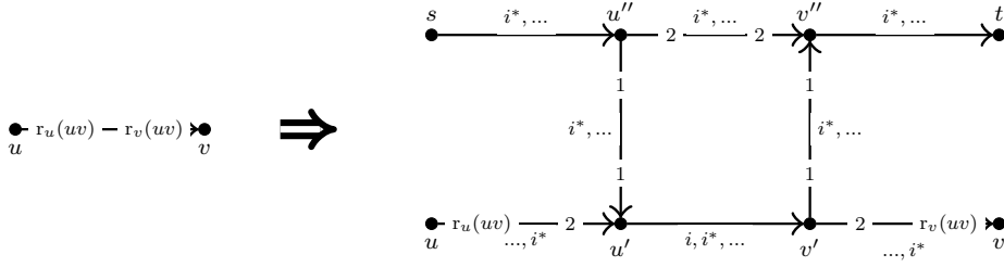
Fig. 9 The gadget ensuring that there are no commodity-specific capacities.
